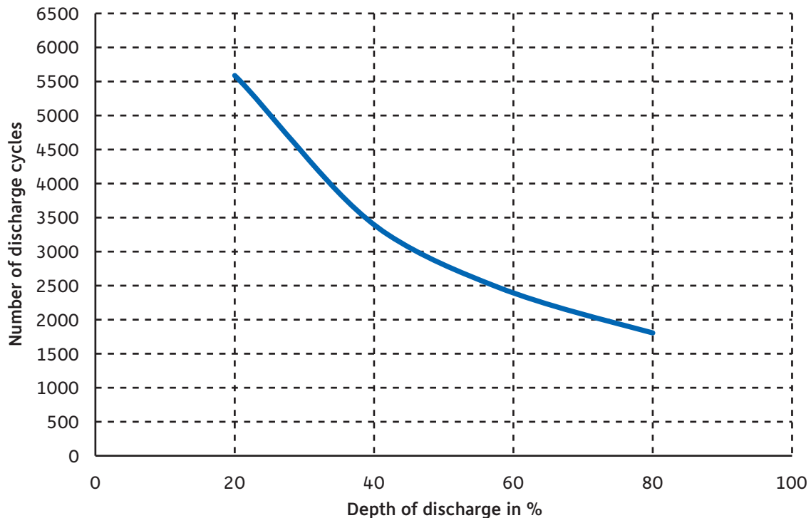
Graph 1, Cycle life vs. DOD of ROBUSTE Series with Ideal Charge Table 1, data of cycle number
